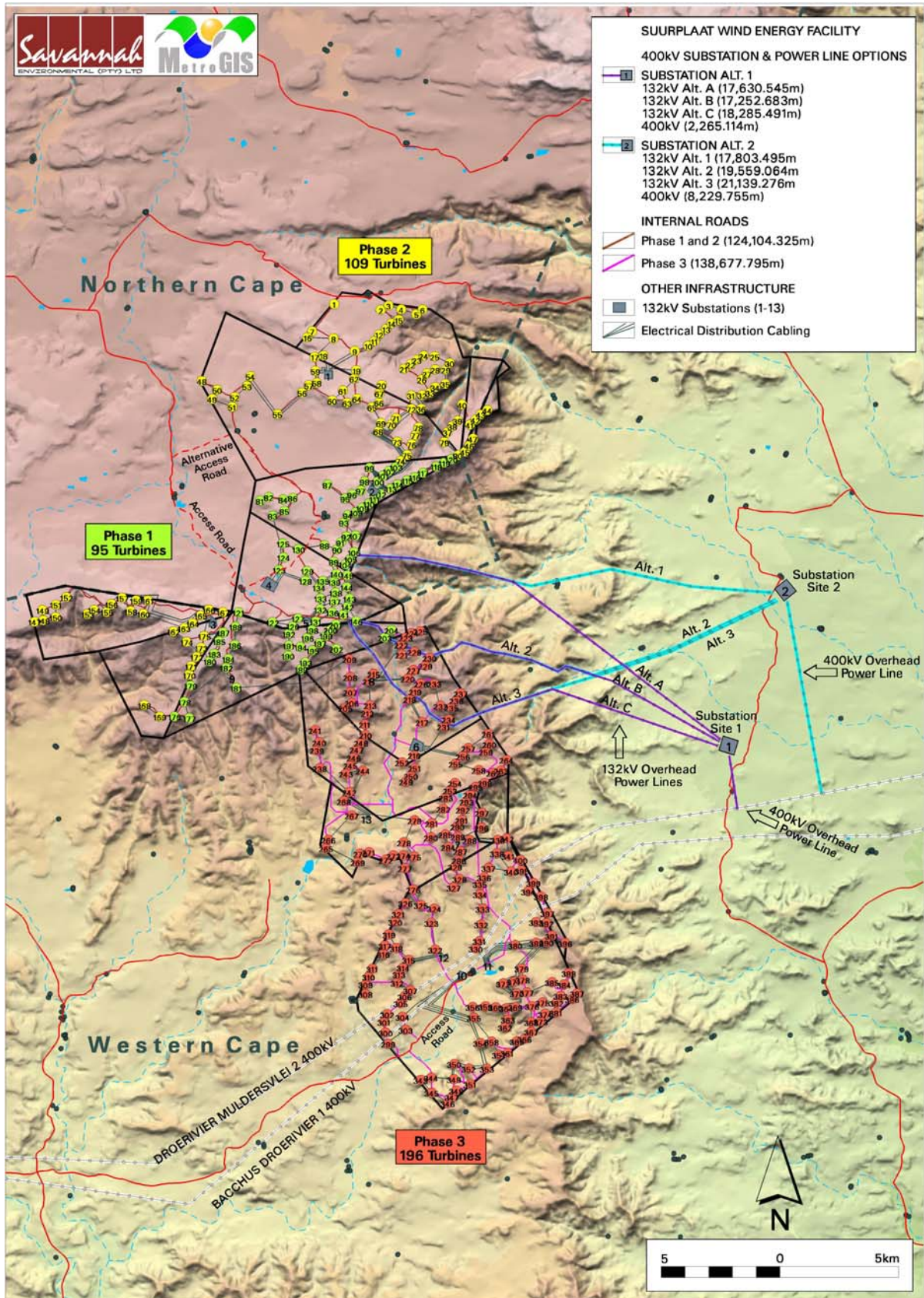
Figure 2.2: Locality map showing provisional wind turbine layout, alternative substation sites, workshop area and alternatives for power lines and external substation linking to the electricity grid
