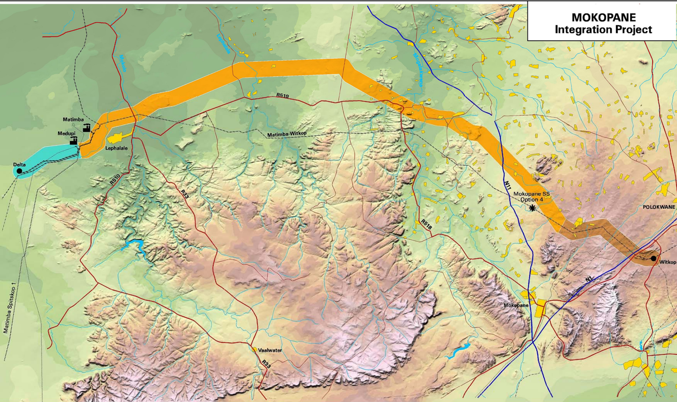
Preferred Transmission Line Alternatives (5km development corridors) and Preferred Mokopane Substation Option
