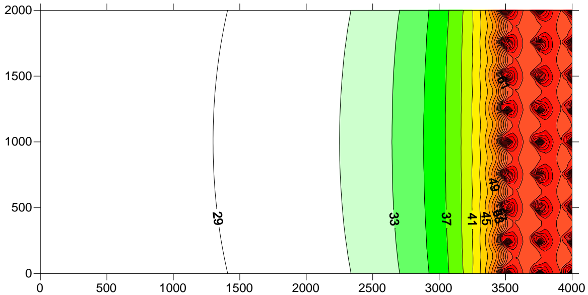
Figure 6-9: 52 WTGs operating in 4 lines (3500m, 3750m, 4000m and 4250m on X-axes) downwind from receptor, all hard ground scenario
